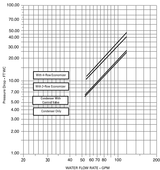
Chart PD-21. Waterside Pressure Drop SCWF/SIWF 35, 38
